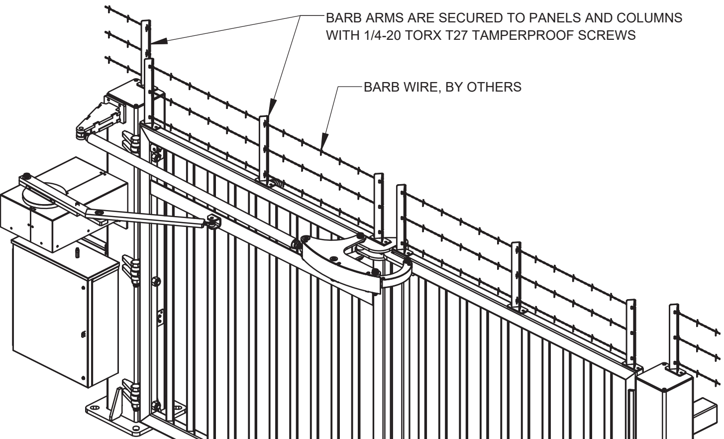
DETAIL M1 - .13 [3] STEEL BARB ARM
