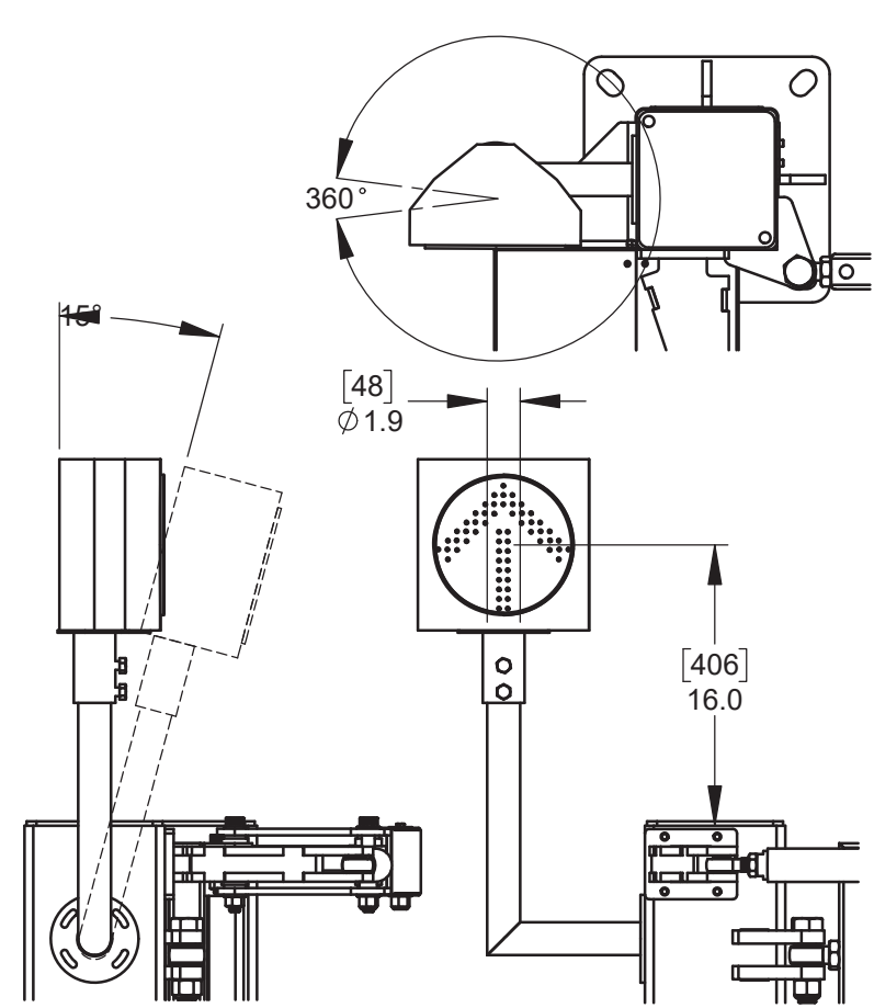
DETAIL I1 - 8" [203] RED / GREEN LED TRAFFIC LIGHT (SIDE MOUNT)
