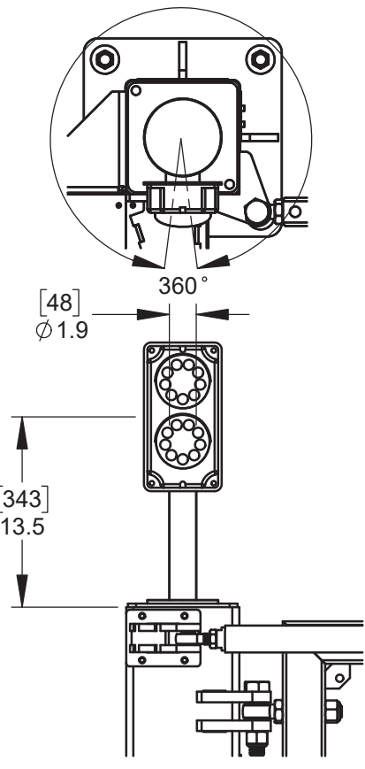
DETAIL J2 - (TOP MOUNT)
