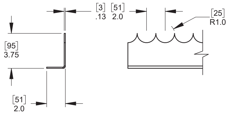
DETAIL L2 - OPTIONAL DRAWBAR STEEL ANTI-CLIMB EDGE
