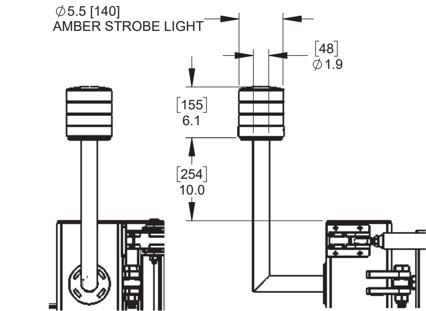
DETAIL K1 - STROBE LIGHT (SIDE MOUNT)
