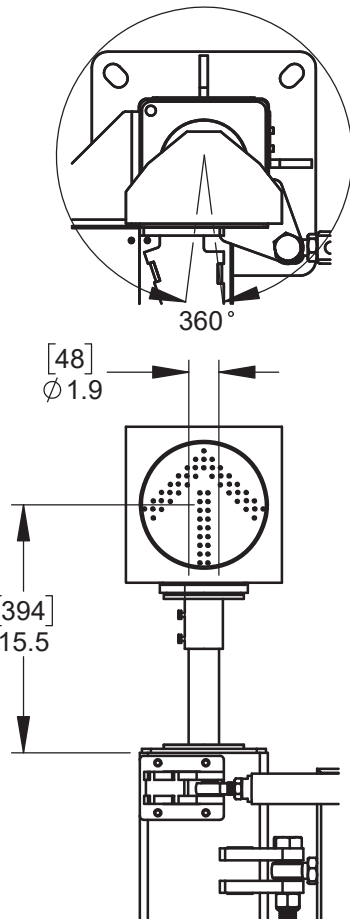
DETEL I2 - (TOP MOUNT)
