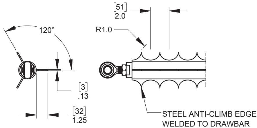
DETAIL L2 - OPTIONAL DRAWBAR STEEL ANTI-CLIMB EDGE
