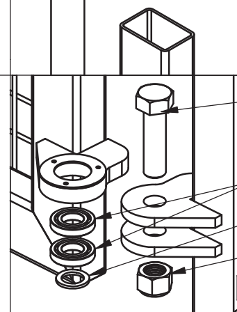
DETAIL C - RAMPART 280 INFILL
