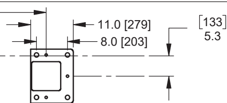
DETAIL B - OPTIONAL CONCRETE TEMPLATE & ANCHOR BOLT KIT
