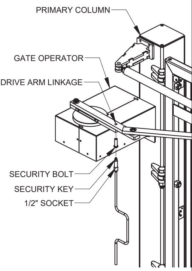
DETAIL H - MANUAL OPERATION RELEASE
