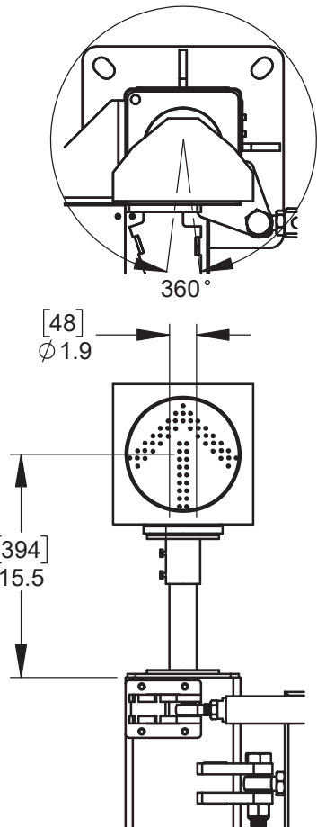
DETIL I2 - (TOP MOUNT)
