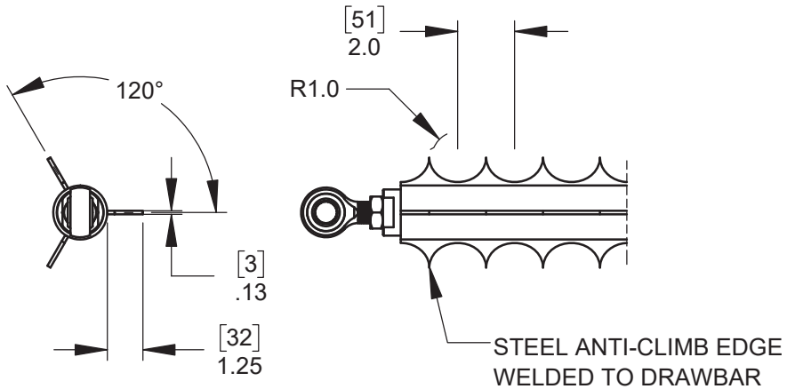
DETAIL L2 - OPTIONAL DRAWBAR STEEL ANTI-CLIMB EDGE
