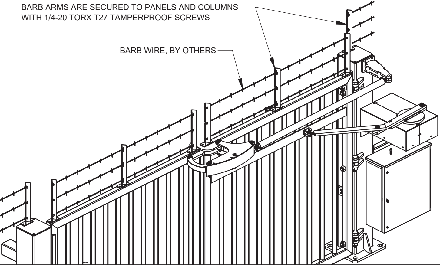
DETAIL M - BARB WIRE ANTI-CLIMB
