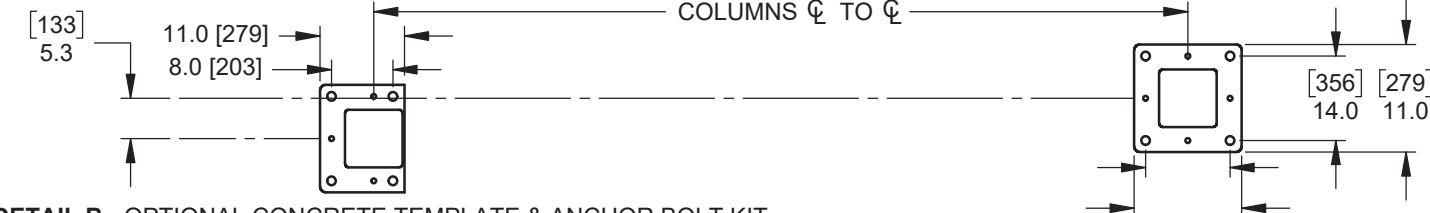
DETAIL B - OPTIONAL CONCRETE TEMPLATE & ANCHOR BOLT KIT
