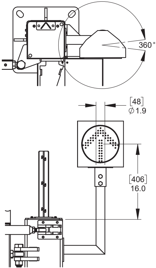
DETAIL K1 - STROBE LIGHT (SIDE MOUNT)
