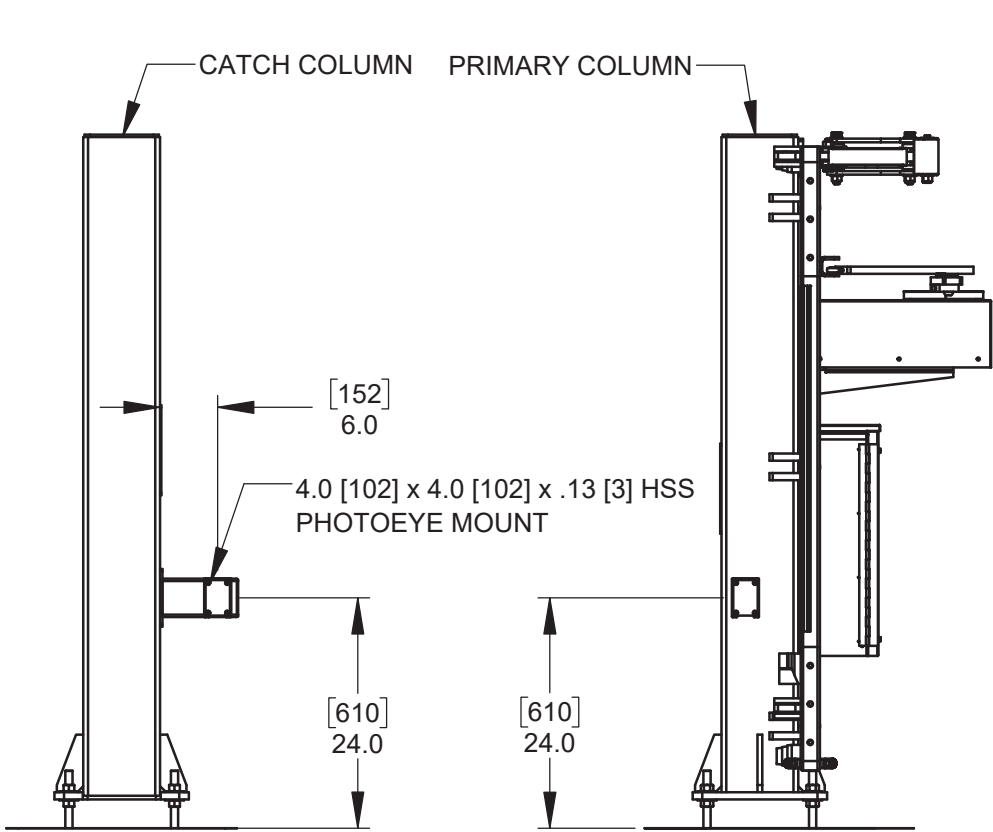
DETAIL G - PHOTOEYES
