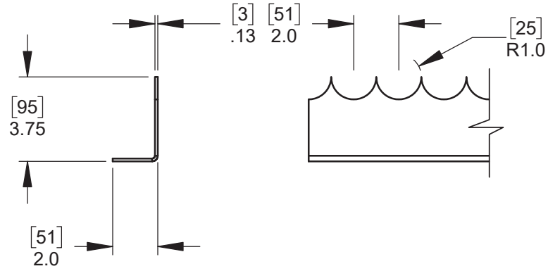
DETAIL L2 - OPTIONAL DRAWBAR STEEL ANTI-CLIMB EDGE
