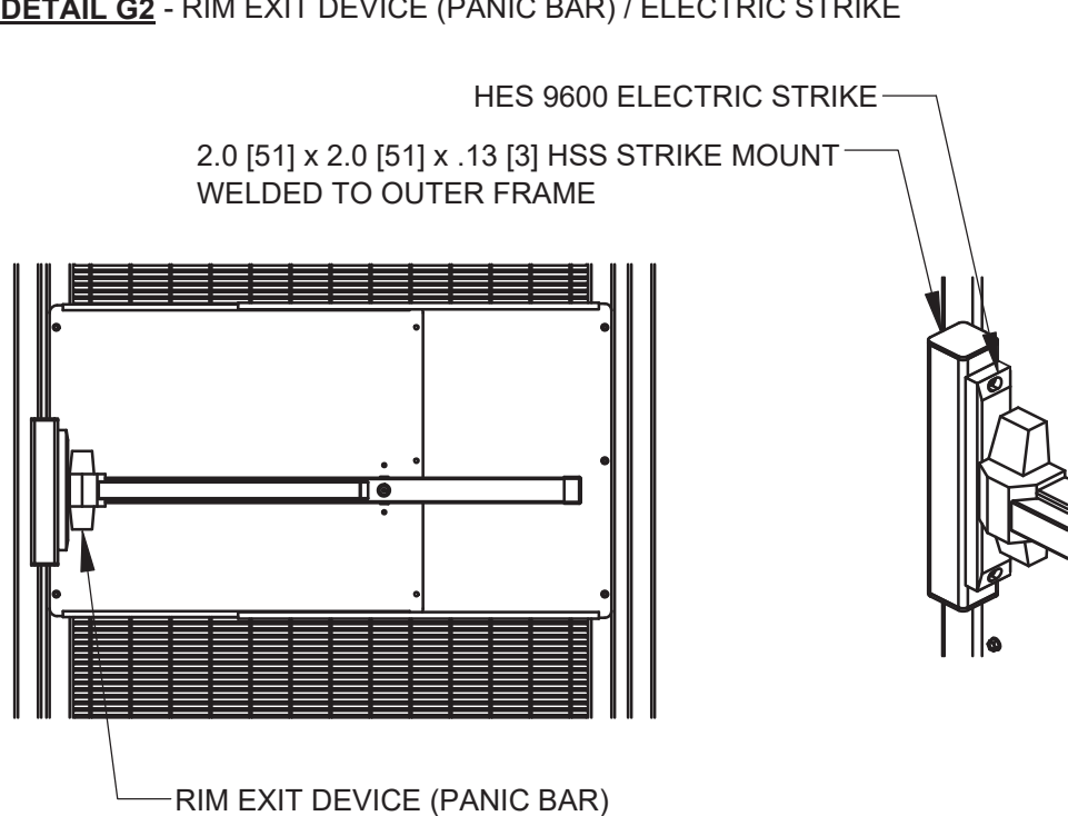
DETAIL G2 - RIM EXIT DEVICE (PANIC BAR) / ELECTRIC STRIKE
