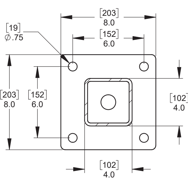
DETAIL B4 - 8" [203] x 8" [203] x .5 [13] BASE PLATE
