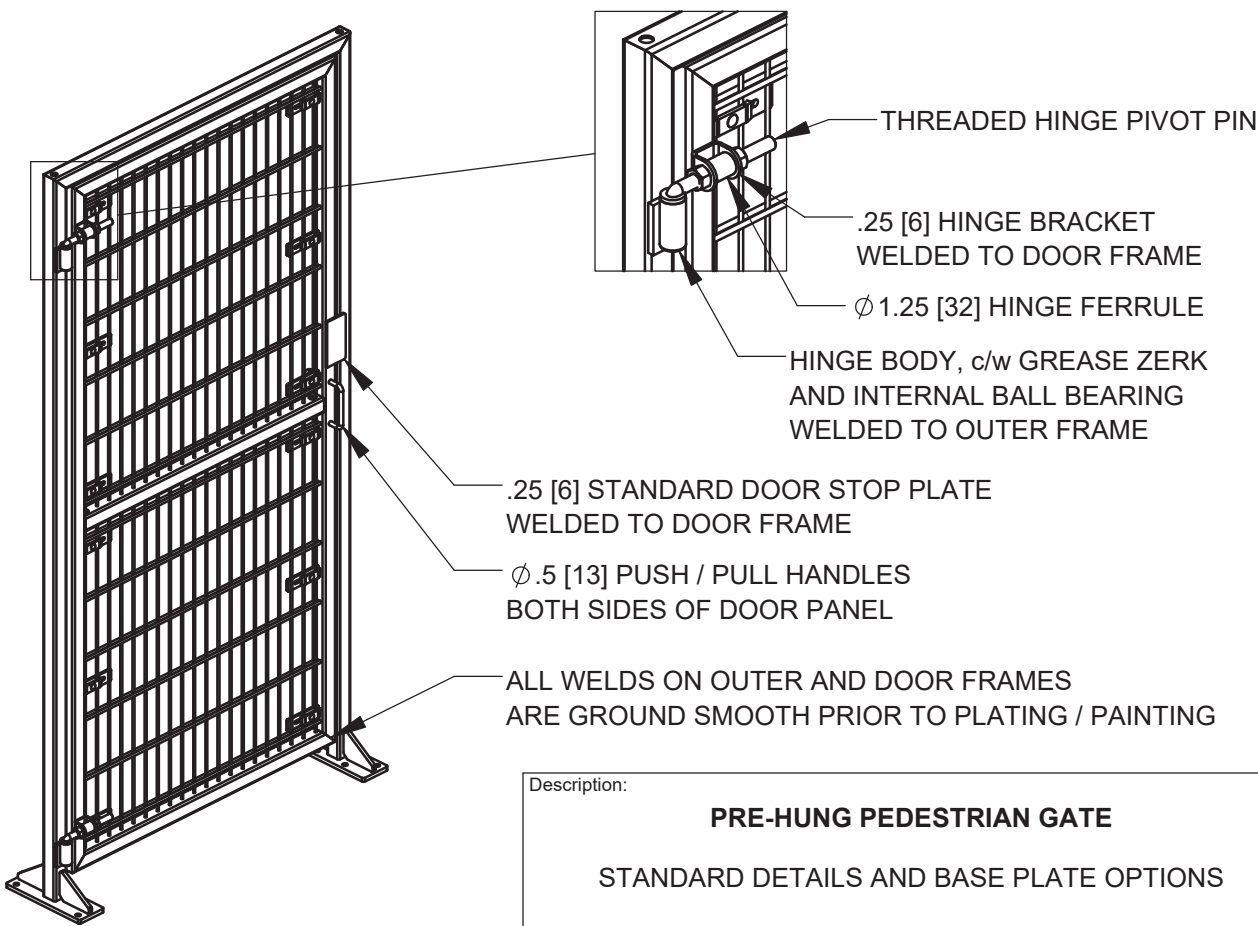
DETAIL D - STANDARD GATE DETAILS
