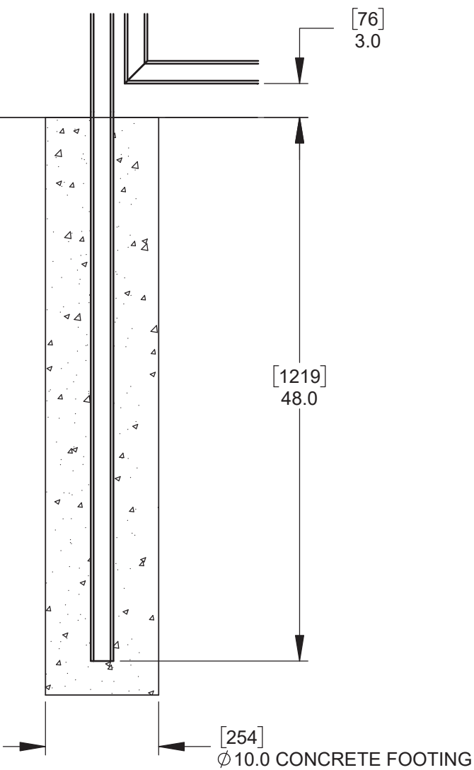
DETAIL C1 - DIG AND SET (CONCRETE FOOTING)
