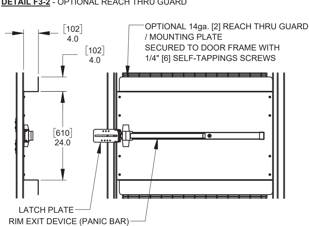
DETAIL F3-2 - OPTIONAL REACH THRU GUARD
