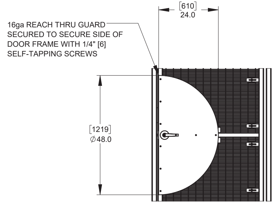
DETAIL J1 - REACH THRU GUARD
