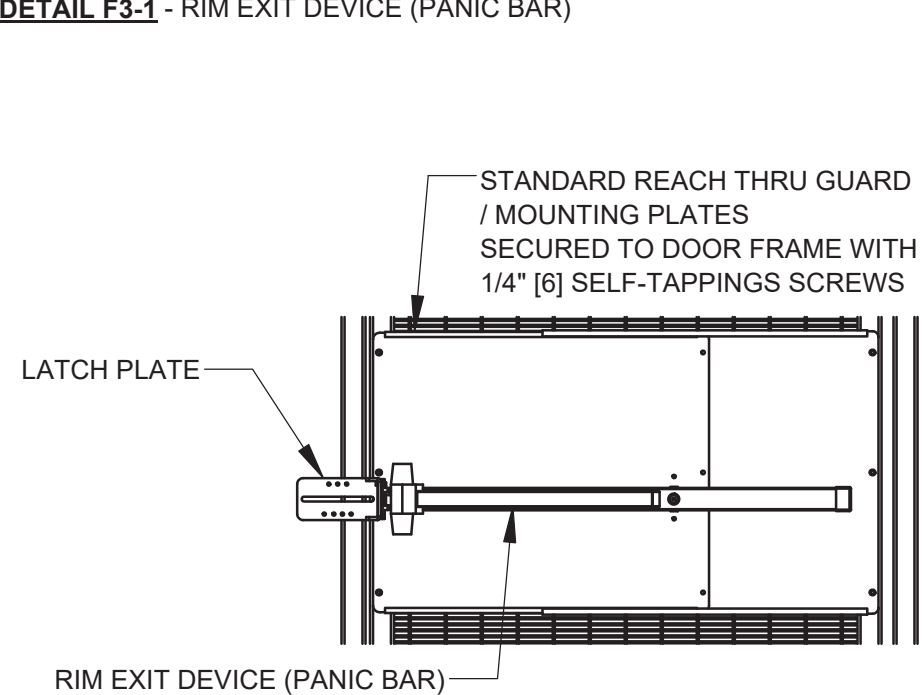
DETAIL F3-1 - RIM EXIT DEVICE (PANIC BAR)
