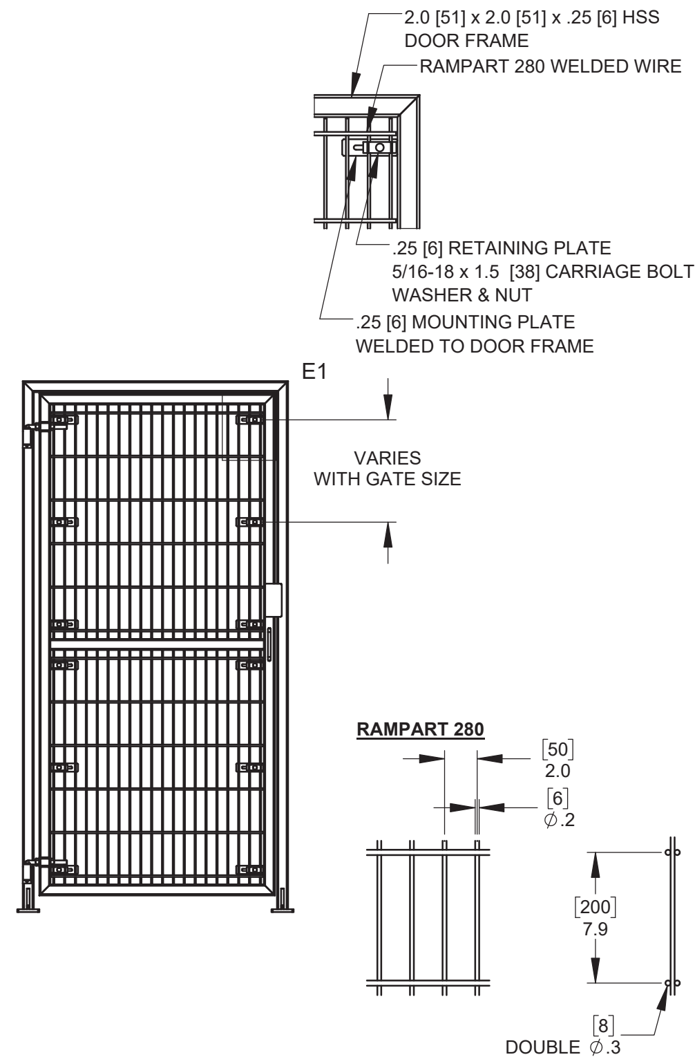
DETAIL E1 - RAMPART 280 WELDED WIRE INFILL
