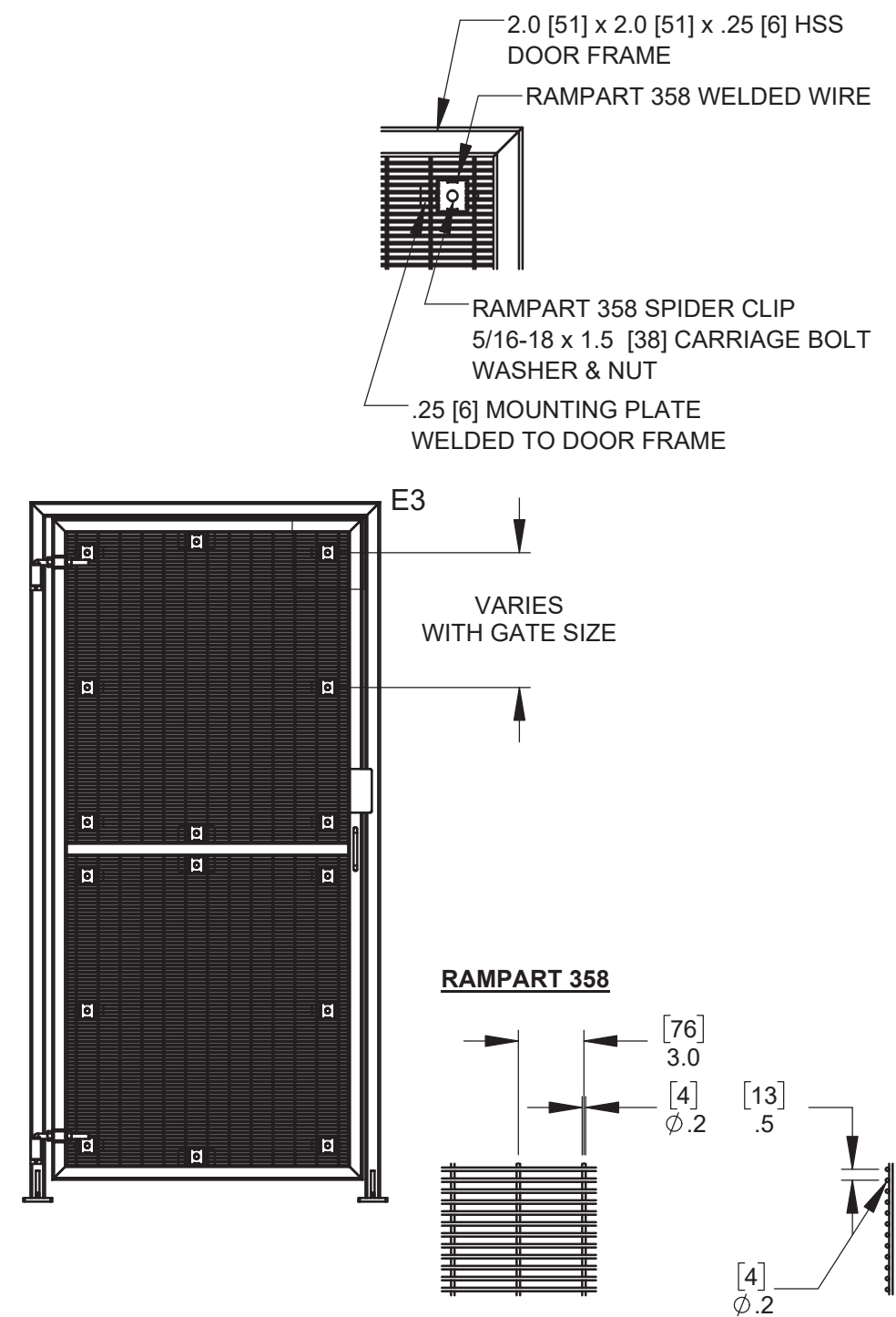
DETAIL E3 - RAMPART 358 WELDED WIRE INFILL
