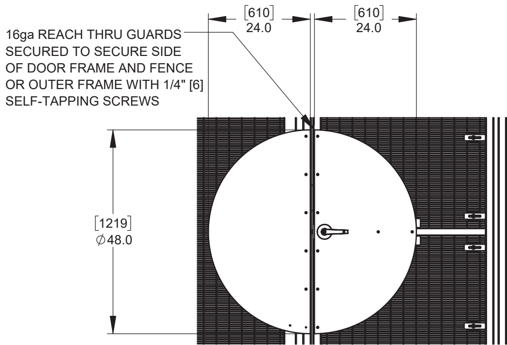
DETAIL J2 - DOUBLE REACH THRU GUARD
