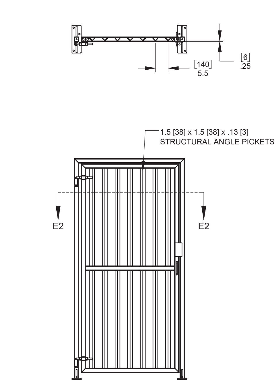
DETAIL E2 - 1.5 [38] x 1.5 [38] x .13 [3] VERTICAL PICKETS
