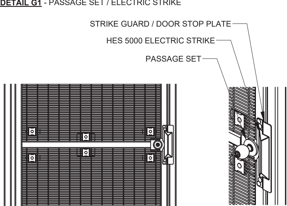
DETAIL G1 - PASSAGE SET / ELECTRIC STRIKE
