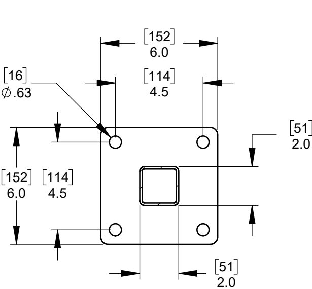
DETAIL B3 - 6" [152] x 6" [152] x .25 [6] BASE PLATE
