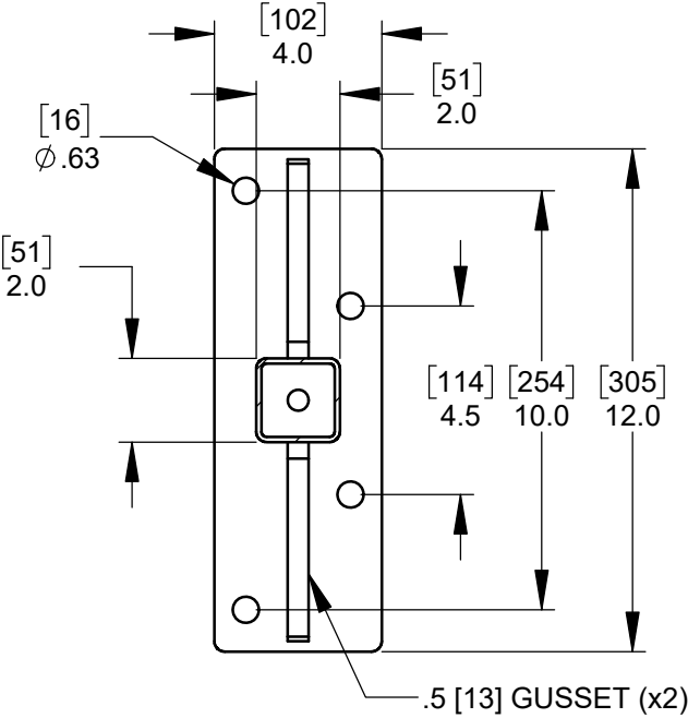
DETAIL B1 - 4" [102] x 12" [305] x .5 [13] BASE PLATE
