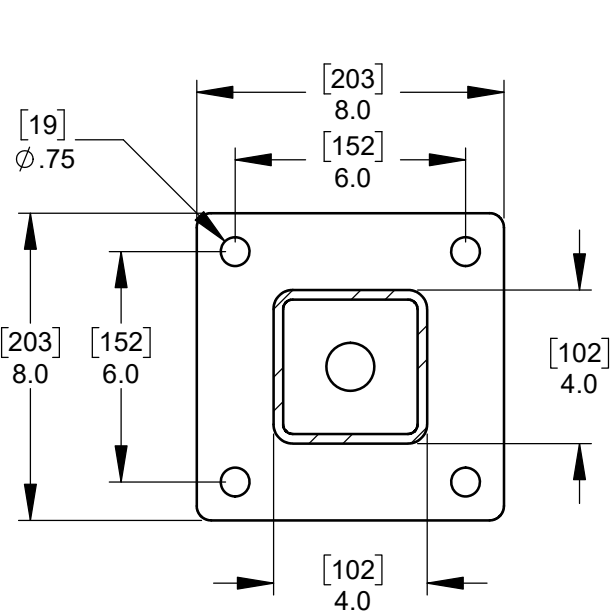
DETAIL B4 - 8" [203] x 8" [203] x .5 [13] BASE PLATE
