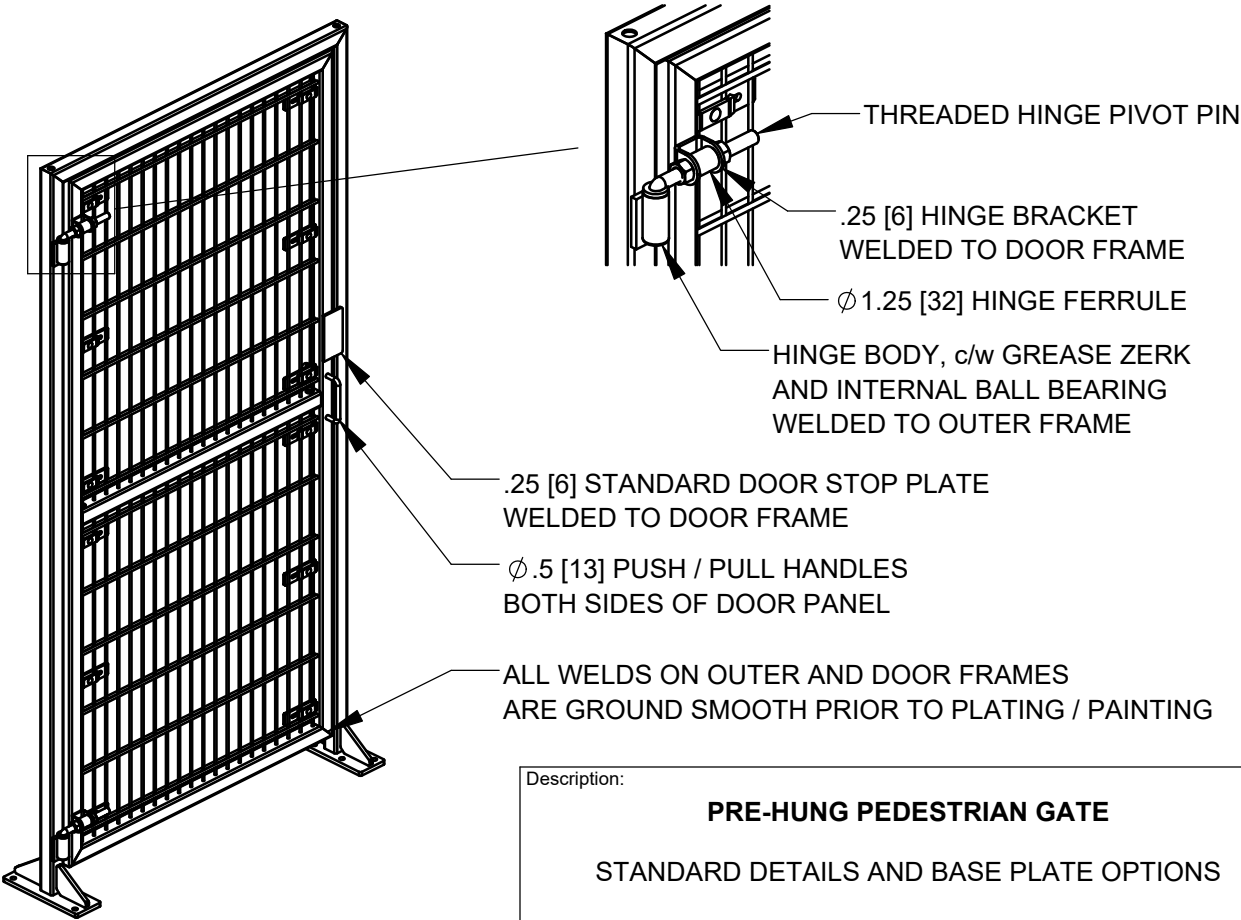
DETAIL D - STANDARD GATE DETAILS
