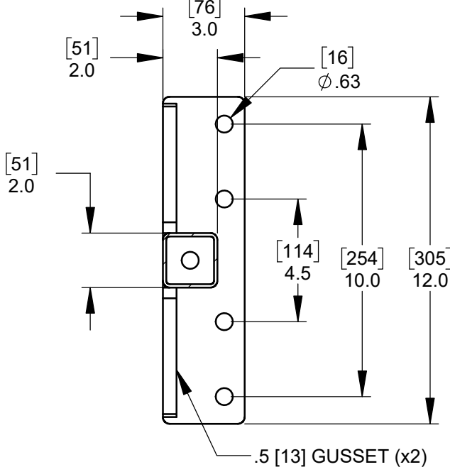
DETAIL B2 - 3" [76] x 12" [305] x .5 [13] BASE PLATE
