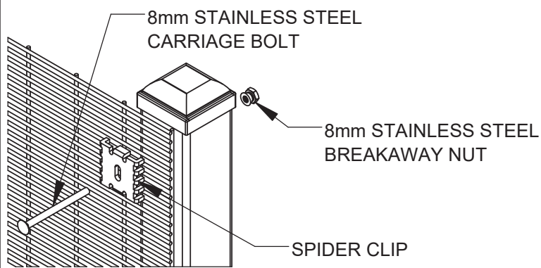
DETAIL A1 - OPTIONAL MOUNTING DETAIL
