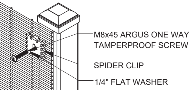
DETAIL A2 - STANDARD MOUNTING DETAIL
